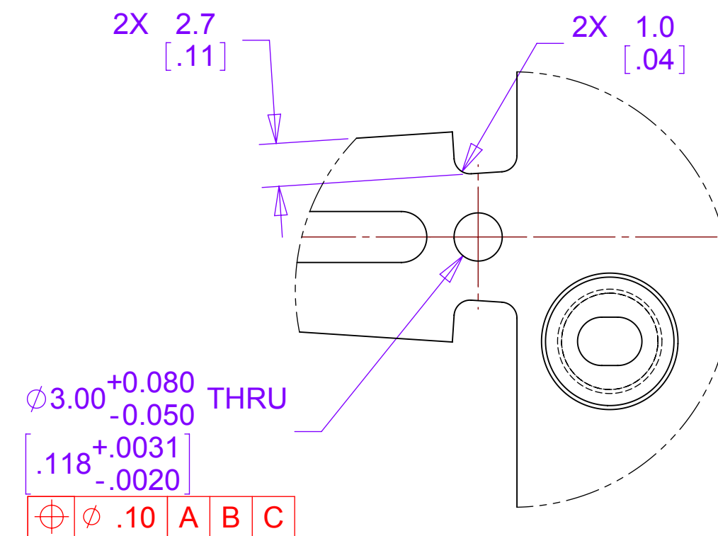
DETAIL D SCALE 3 : 1
